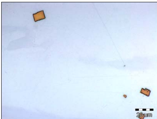
Hard titanium carbonitrides in the stabilised steel Photo: Acroni, Jesenice (SI)
