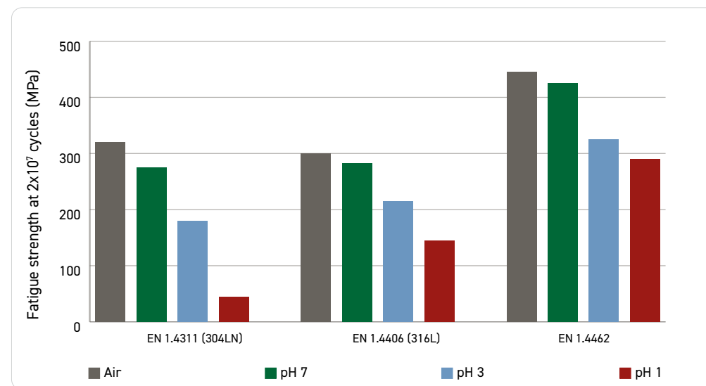
Figure 3.13 Fatigue strength of some stainless steels obtained by rotating bending at 40°C, 100Hz, in air and in 3%NaCl solutions at different pH (Ref 3.18)
