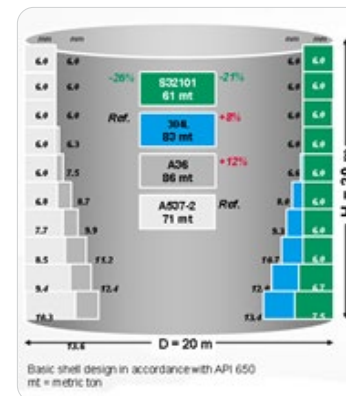
Figure 6.2 Thickness reduction achieved by duplex stainless steels (Ref 6.13.7)
