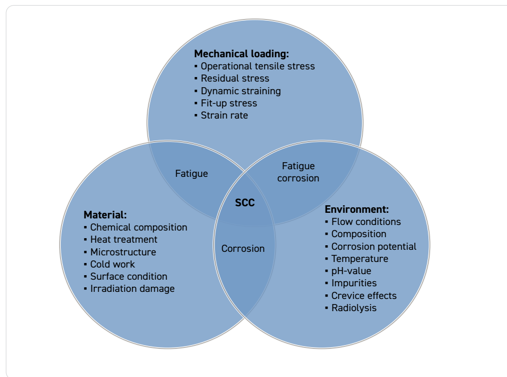
Figure 3.9 Factors effecting Stress Corrosion Cracking. ( Ref 3.15 )
