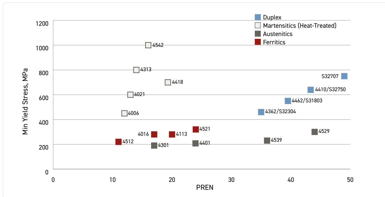
Figure 3.1 Minimum Yield Stress vs. Pitting Corrosion Resistance (section 3.2).
