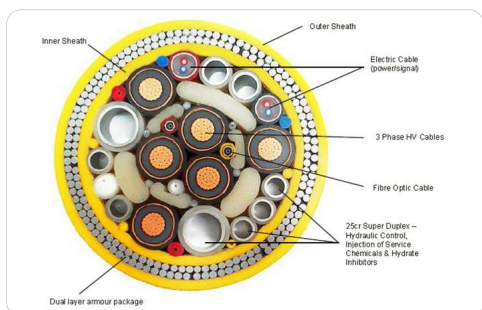
Cross section of an umbilical (Ref 6.10.9)
