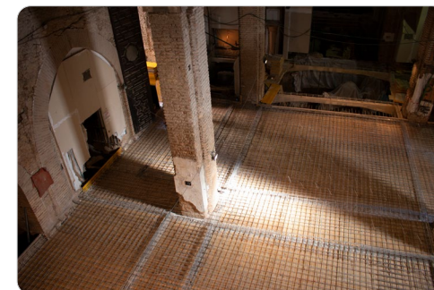
Reinforcing stainless bar in the floor of the Santa Catalina church in Spain Picture courtesy of Cedinox
