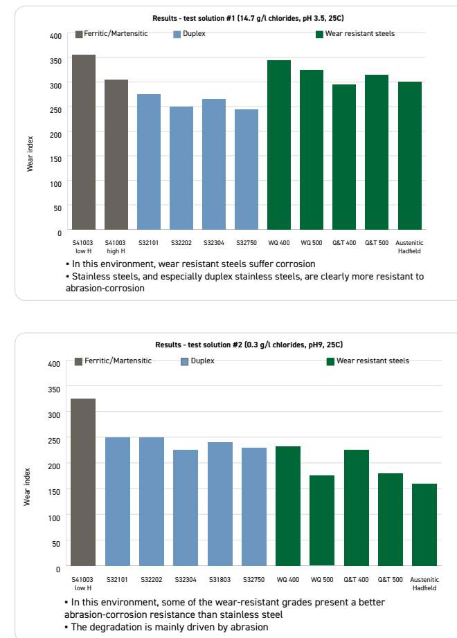
Figure 3.15 Wear resistance of Duplex vs Wear resistant Steels Note: The higher the wear index, the higher the abrasion-corrosion
