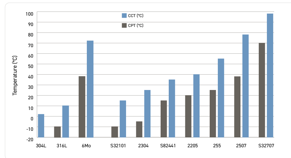
Figure 3.8 CPT* and CCT* for austenitic and duplex stainless steel (Evaluated in 6% ferric chloride by ASTM G48). (Ref 2.1)
