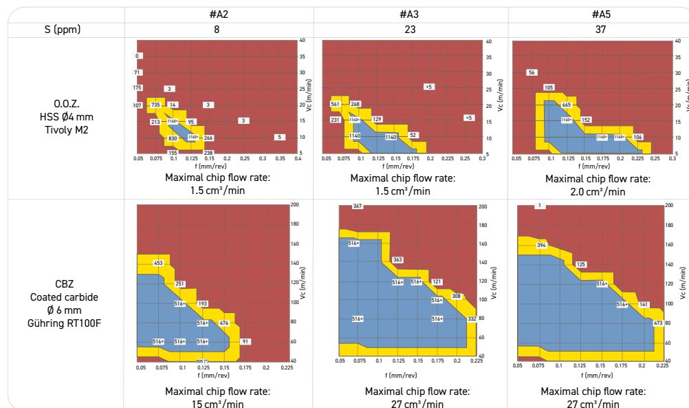
Figure 7.2.1 Optimum chip breakability vs Sulphur content for High Speed Steel and for Coated Carbide cutting tools (Ref 7.2.2)
