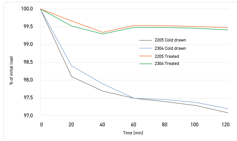
Figure 5.7 Load relaxation of duplex stainless steels (Ref 5.12)
