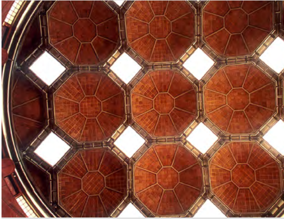
Figure 6: Internal view of the VIP dome
