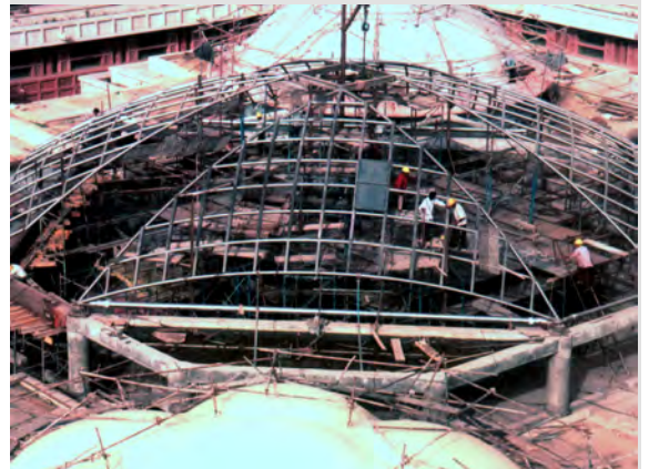
Figure 8: Erection of the focal dome
