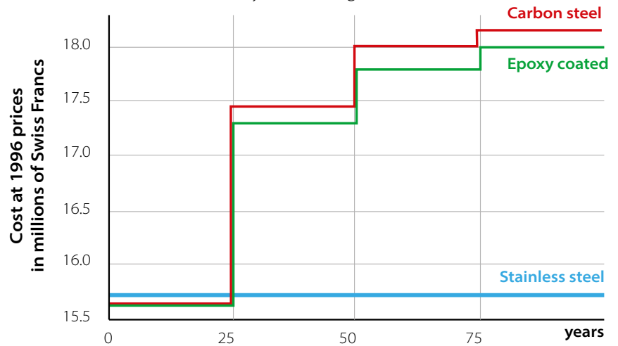
Data from TR51 Guidance on the use of stainless steel reinforcement. Concrete Society
