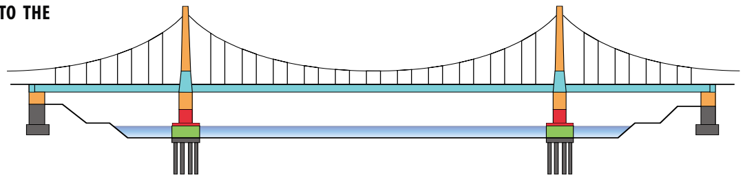
Atmospheric zone Deck and De-icing Salt Spray zone Submerged zone Splash zone Embedded zone
