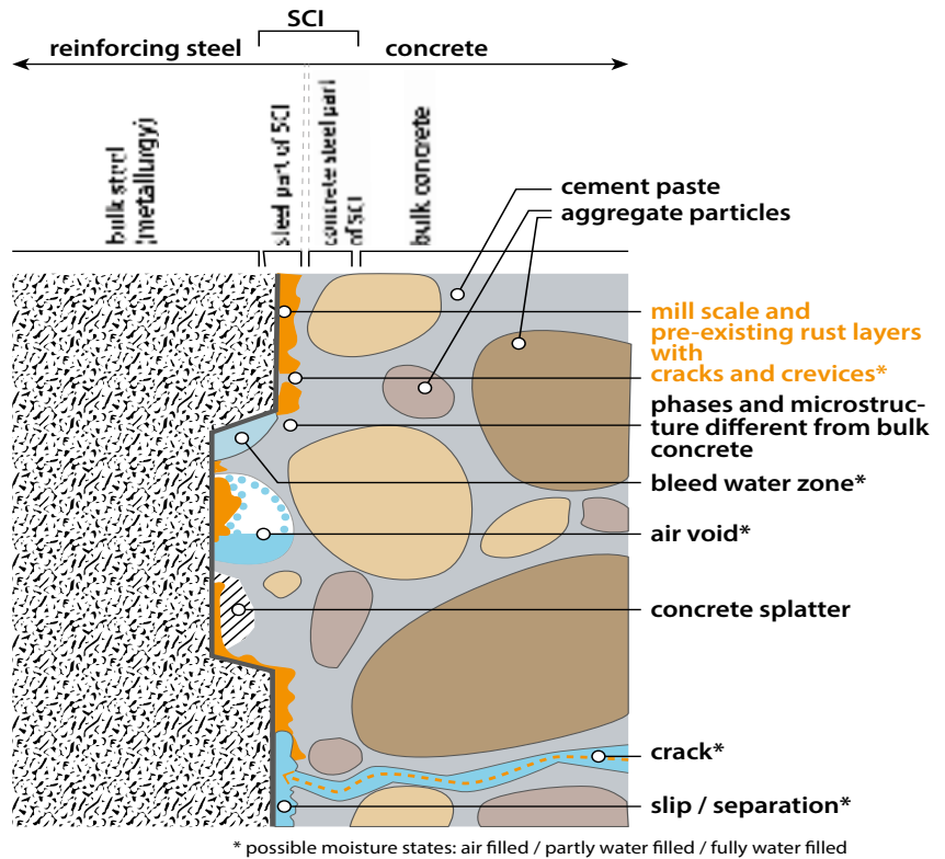
Source: Figure from The Steel Concrete Interface Publication: Materials and Structures Author: Ueli M. Angst et al Publisher: Springer Nature Feb 27, 2017
